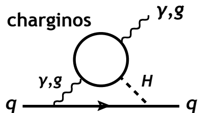
Barr-Zee type diagram
