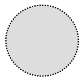
s-wave
