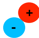
p-wave
