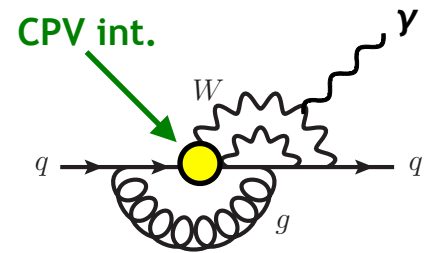
3-loop diagram (e.g. Standard model)
